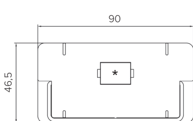
RMMV12X - RMMV16X
