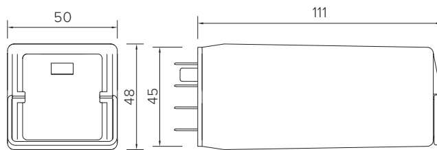
RGMV17X
